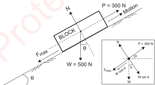
(b) Block just move upwards
