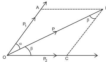
Fig. 1.10: Non-orthogonal components
