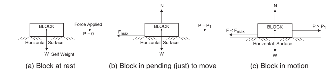
Fig. 3.2: Limiting friction
