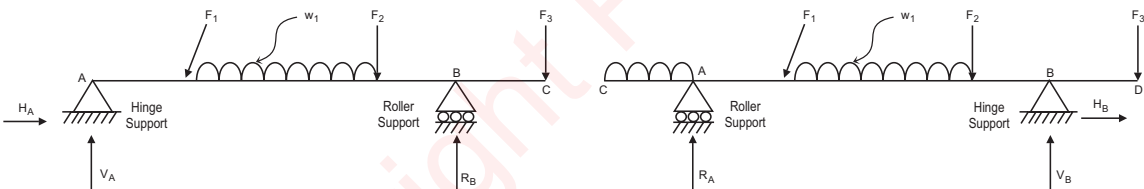
Fig. 2.12: Overhang beam
