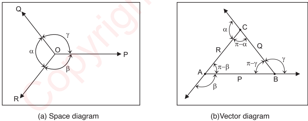
Fig. 2.5: Lami's theorem
