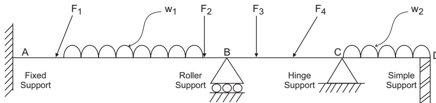
Fig. 2.14: Continuous beam
