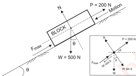
(a) Block just move downwards
