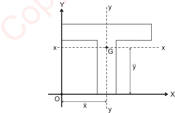
Fig. 4.2: Axis of reference
