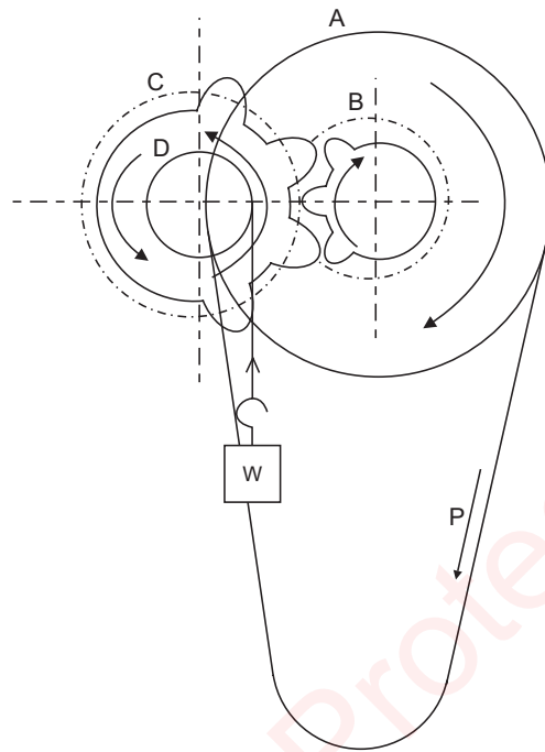
Fig. 5.9: Geared pulley block
