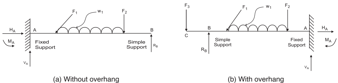
Fig. 2.13: Propped cantilever
