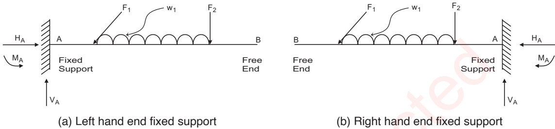
Fig. 2.11: Cantilever beam
