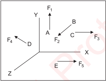
Fig. 1.3: Coplanar force system and non-coplanar force system
