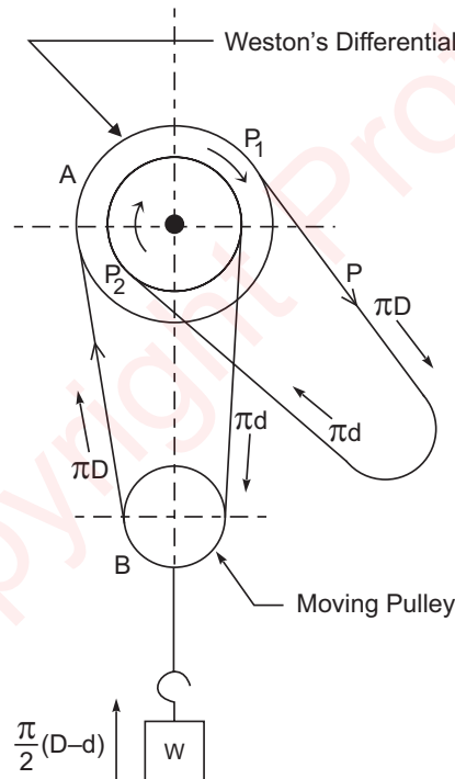
Fig. 5.8: Weston's differential pulley block
