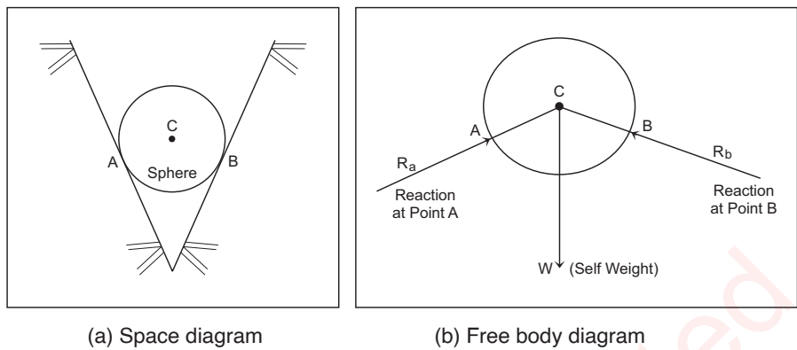
Fig. 2.4: A sphere resting in V-shaped groove
